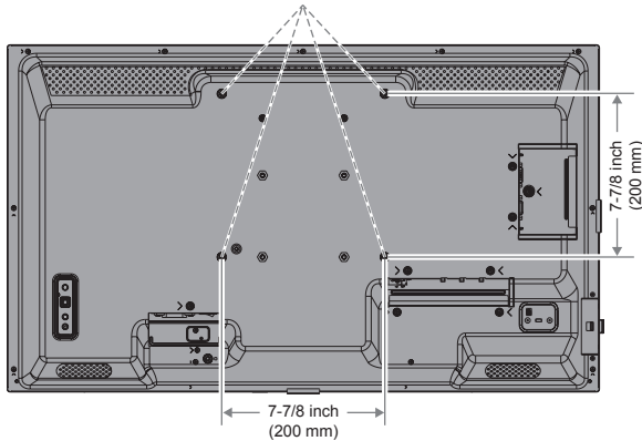
Mounting Interface (M4)
