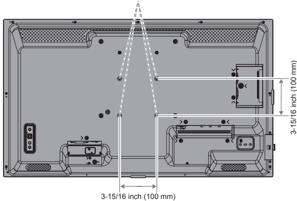
Mounting Interface (M4)
