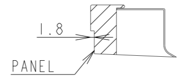
SECTION C-C SCALE 1:2
