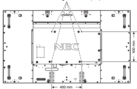
VESA-montage-interface (M8)
