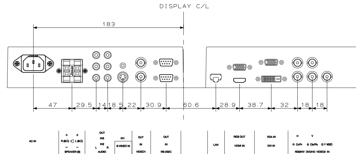
I/O TERMINAL
