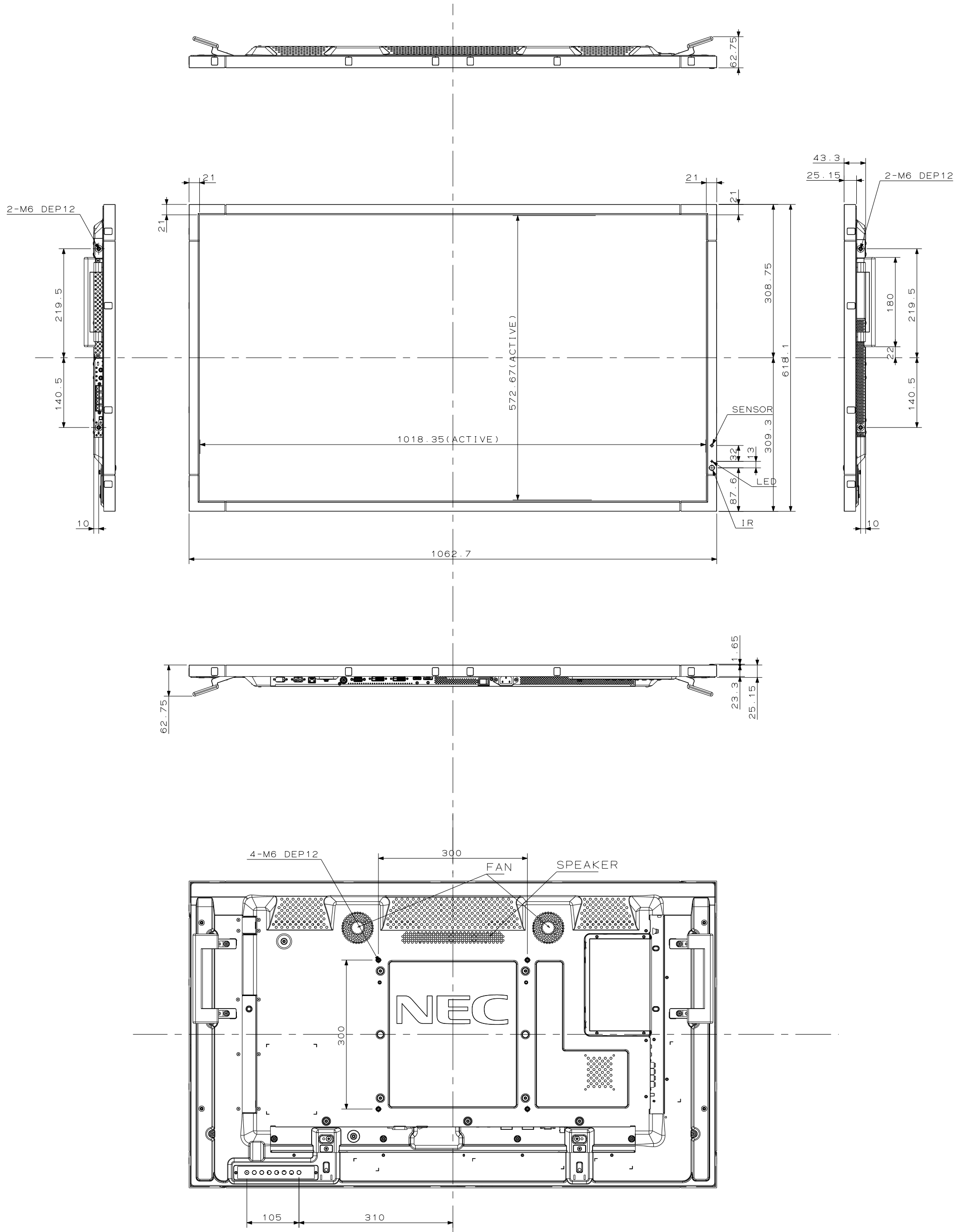
X461S OUTLINE DRAWING 2011/04/26
