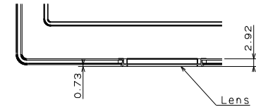
Detail C Scale 1/1
