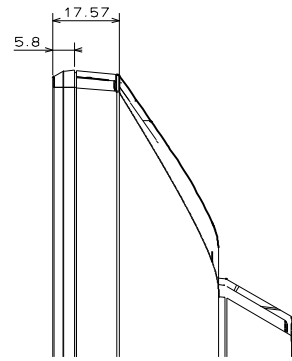
Detail D Scale 1/1
