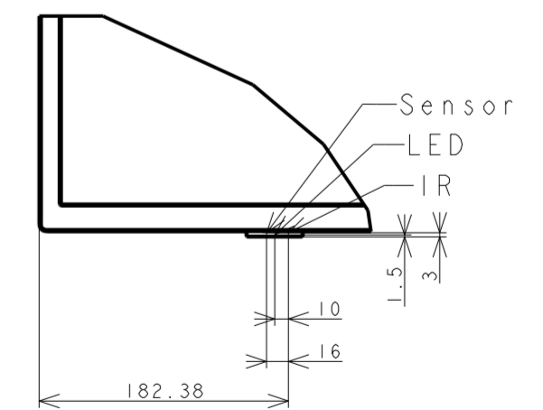
DETAIL B SCALE 1:5
