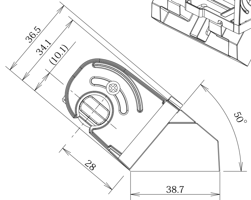
KT-RC3 Sensor Unit with spacer outline drawing 2018.11.22 NEC Display Solutions, Ltd.
