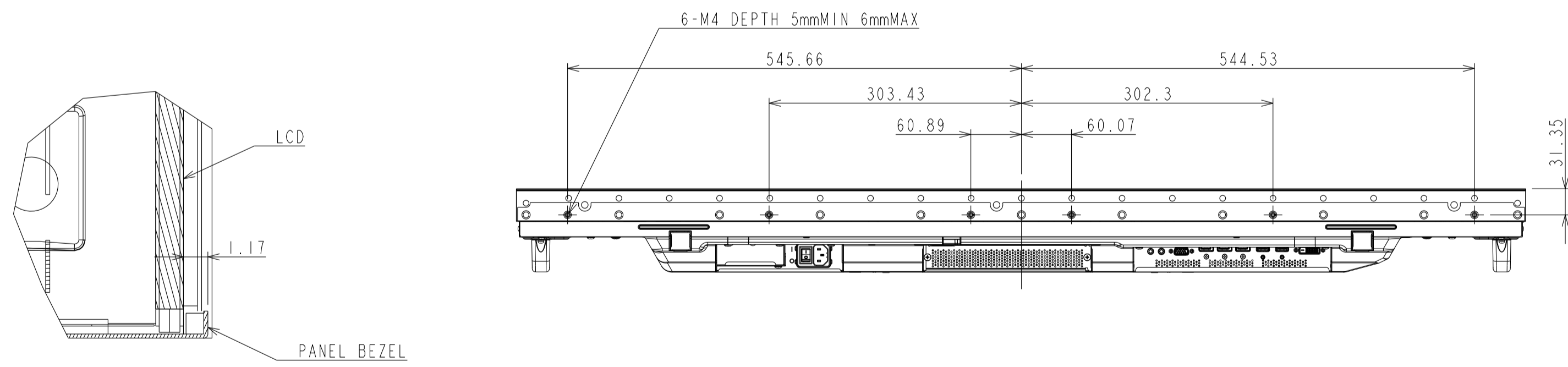
SECTION A-A(BOTTOM) SCALE 5/1
