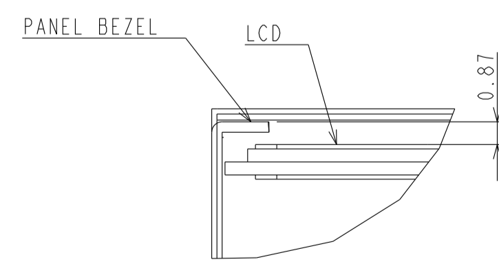
SECTION B-B SCALE 5/1
