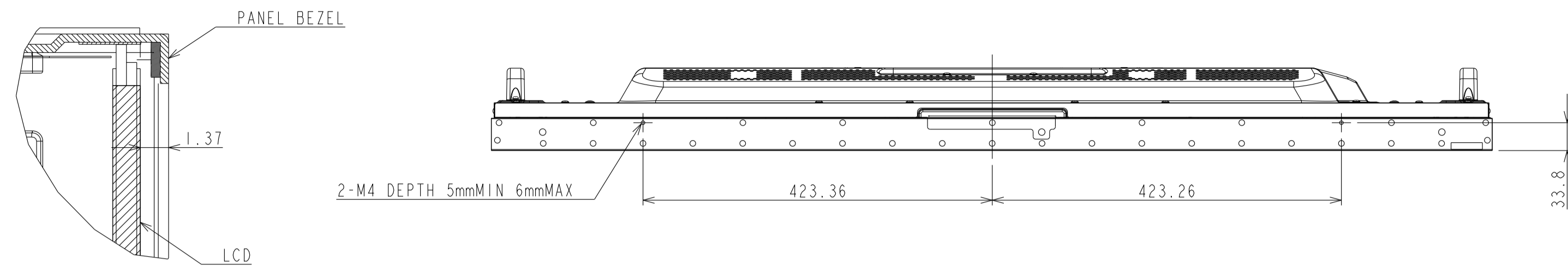
SECTION A-A(TOP) SCALE 5/1
