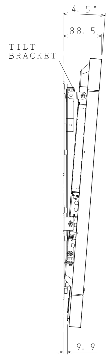
TILT MODE
