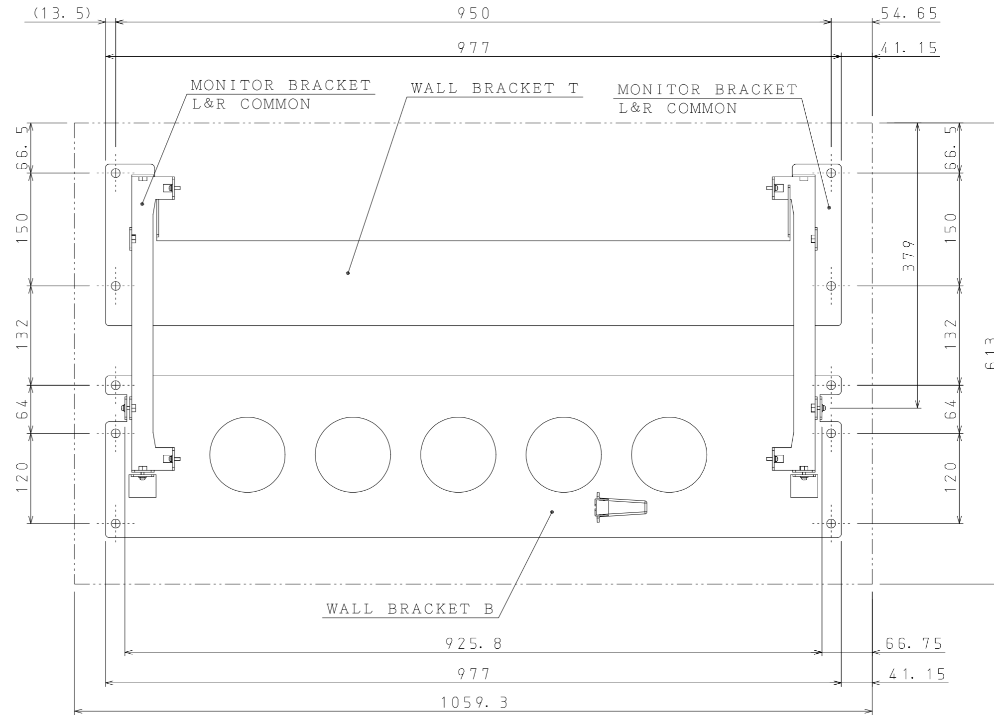
MOUNT MODE
