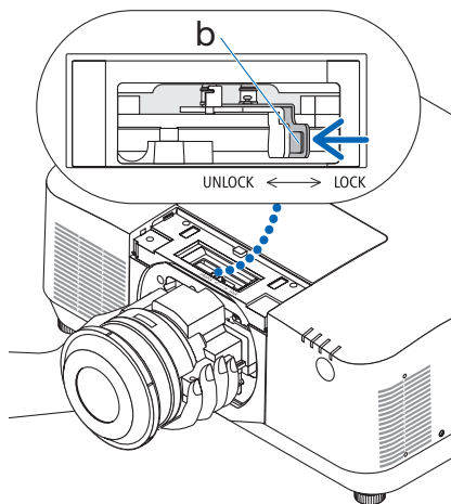
b：鏡頭鎖定桿
