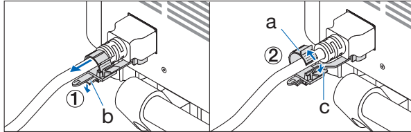
a: Clammer / b: Knob (power cord stopper) / c: Knob (clammer)
